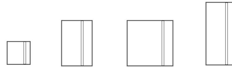
F128C/BAX184 ottone - brass F128C/MRX184 inox L 54 H 54 P 6 cm F128H/BAX239 ottone-brass F128H/MRX239 inox L 74 H 104 P 6 cm F128B/BAX278 ottone-brass F128B/MRX278 inox L 104 H 104 P 6 cm F128M/BAX385 ottone-brass F128M/BAX385 inox L 74 H 144 P 6 cm
