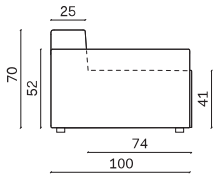
With 52cm-high arm
