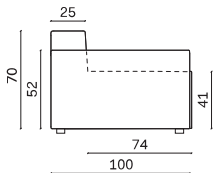
With 52cm-high auxiliary arm
